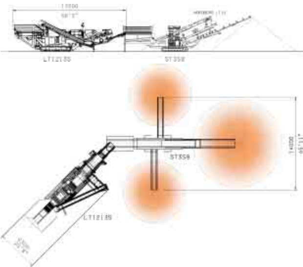
Lokotrack LT1213S + ST358 mobile screen, open circuit
